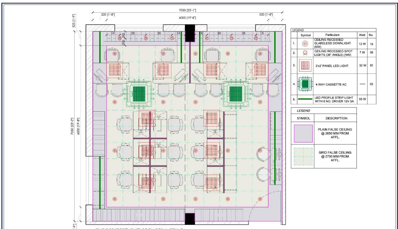
4TH FLOOR SECRETARIATE ROOM RCP. & CEILING ELECTRICAL LAYOUT SCALE 1:35
